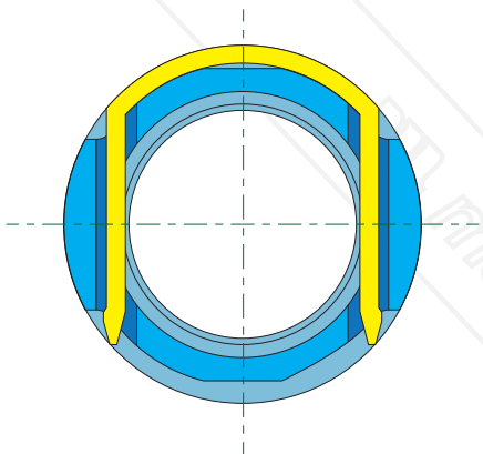
Cross-Section Of a Flushfit Fitting with Staple In-Situ
